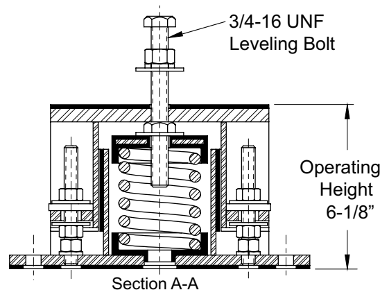
SRMT-1 (Top bolt): Overall dimensions
