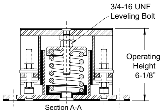
SRMF-1 (Flat top): Overall dimensions
