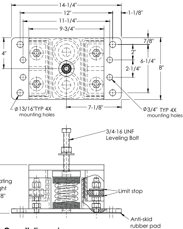
MWT-2: Overall dimensions
