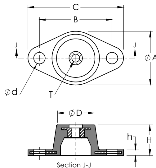
Mount dimensions in inches (in)
