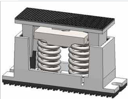
Flat Surface Top Assembly with Rubber
